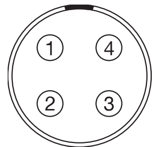
Figure: Front Face of the SYNC (Video Sync) Connector (Looking at the Camera)
