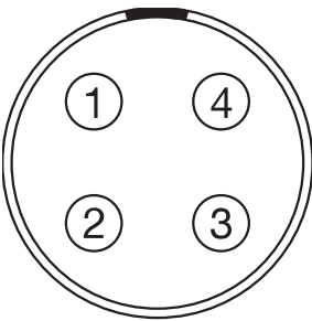
Figure: Front Face of the SYNC (Video Sync) Connector (Looking at the Camera)
