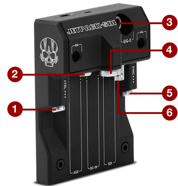
Figure: DSMC2 Jetpack-SDI Expander
