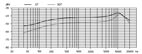
Frequency response ME 104/ME 105
