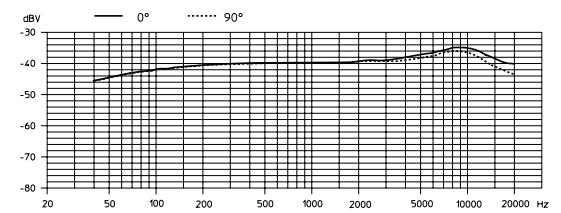
Frequency response ME 102
